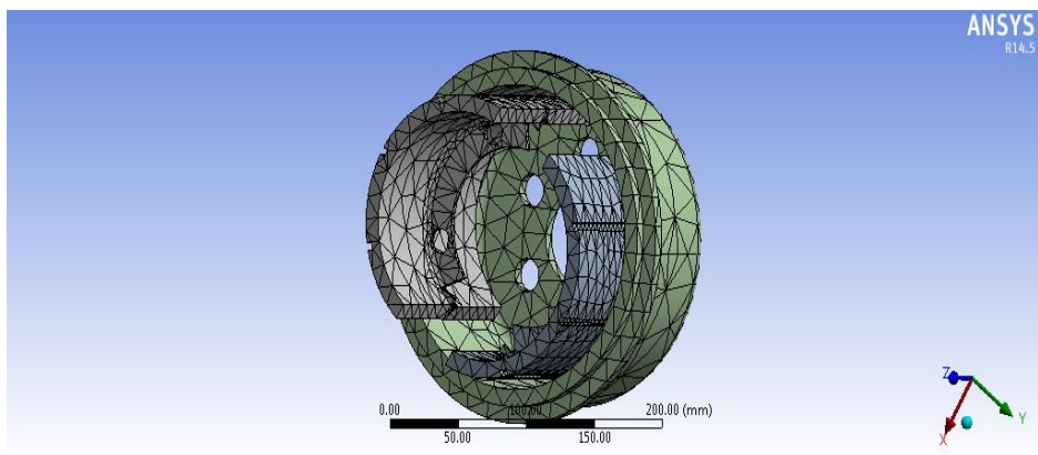
Fig.5: Meshing model.
