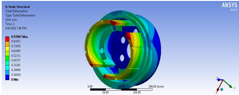
Fig. 6: Deformation.
