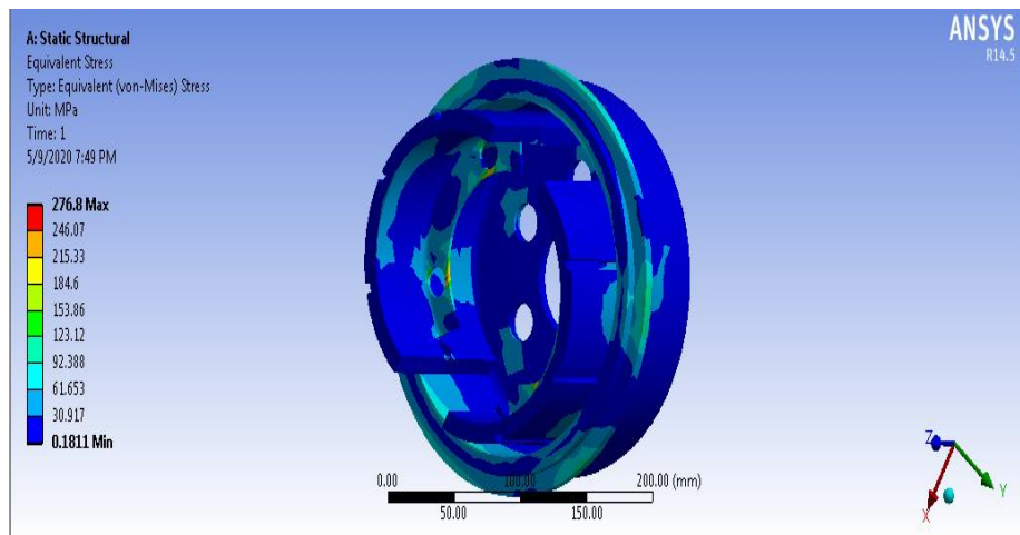
Fig. 7: Stress.
