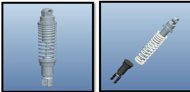
Fig. 2:(a) Solid model of suspension system. (b) Exploded view of suspension system.
