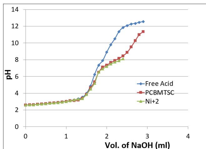
Figure 13. pH titration curves of Ni(II)-PCBMTSC binary system in 70% v/v DMF -water medium at 303K and 0.1M(KNO 3 ) ionic strength
