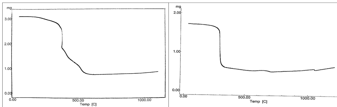
Fig. 1. Thermogram of Ni(II)-PCBMTSC complex Fig.2. Thermogram of Cu(II)-PCBMTSC complex
