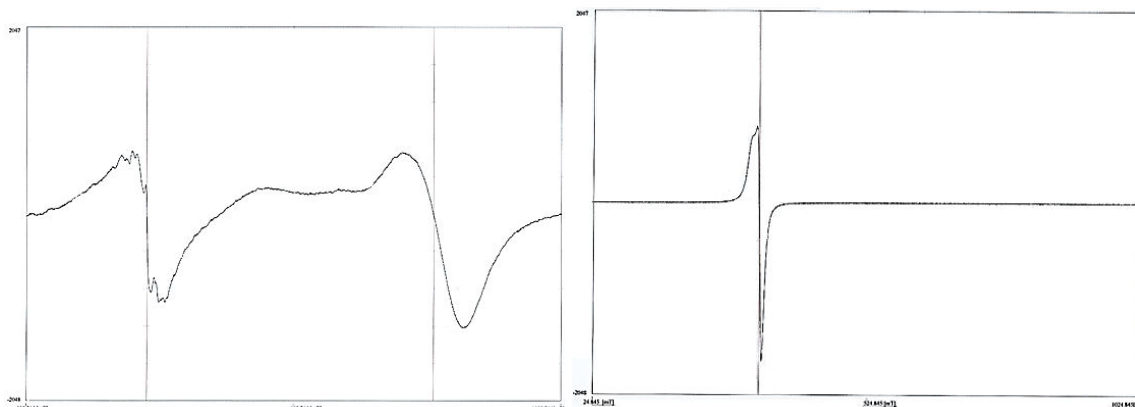
Fig. 5. ESR of Ni(II)-PCBMTSC complex Fig. 6. ESR spectrum of Cu(II)-PCBMTSC complex
