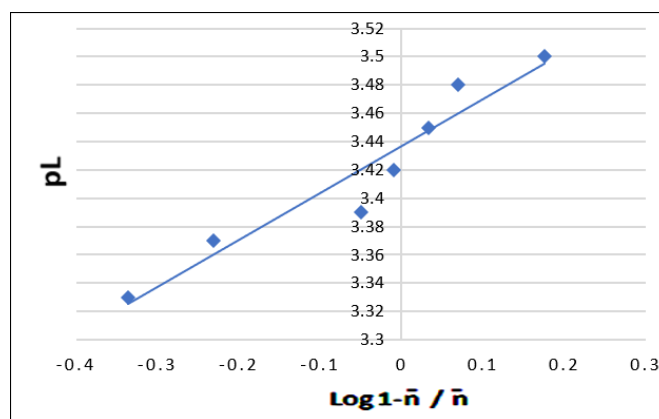
Figure15. Plots of \text{Log}(1-n)/n Vs pL of Ni(II)-PCBMTSC in 70% v/v DMF–Water medium
