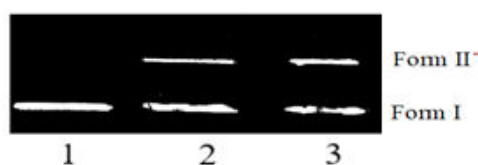
Figure 19. Photocleavage studies of pBR322 plasmid DNA by metal complexes. Lane 1, DNA control, Lane 2, DNA+ complex 1, Lane 3, DNA+ complex 2 respectively
