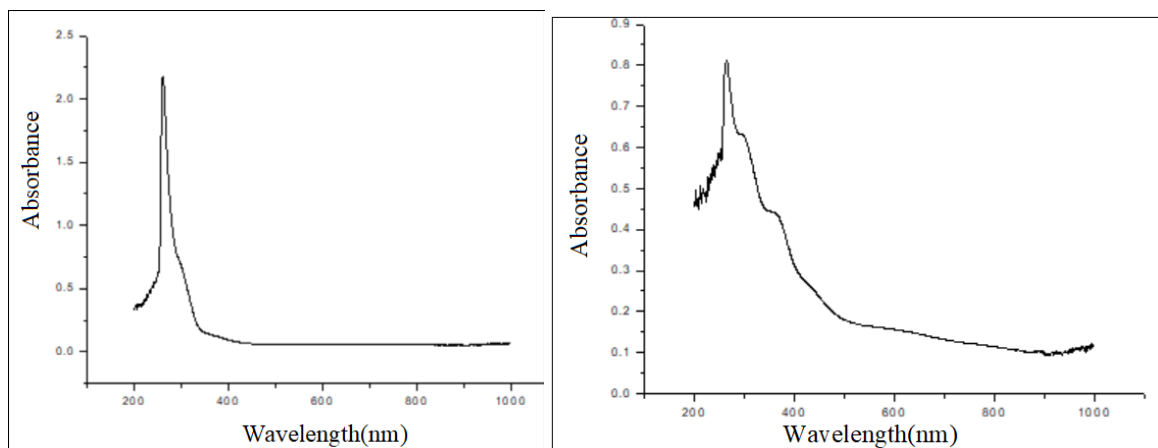
Fig.7. UV-Visible spectrum of Ni(II)-PCBMTSC Fig.8. UV-Visible spectrum of Cu(II)-PCBMTSC
