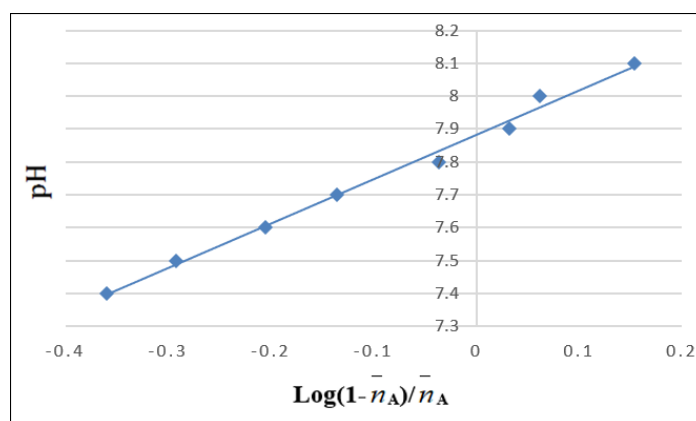
Figure 14. Linear Plot of Log [(1-\bar{n}_A)/\bar{n}_A] Vs pH
