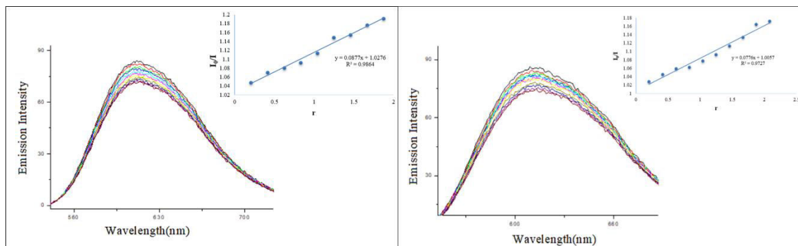
Fig. 17: Emission spectra of EB-DNA, in increasing concentrations of a. Ni(II)-PCBMTSC complex b. Cu(II)-PCBMTSC complex (Inset: linear stern -Volmer quenching curves)
