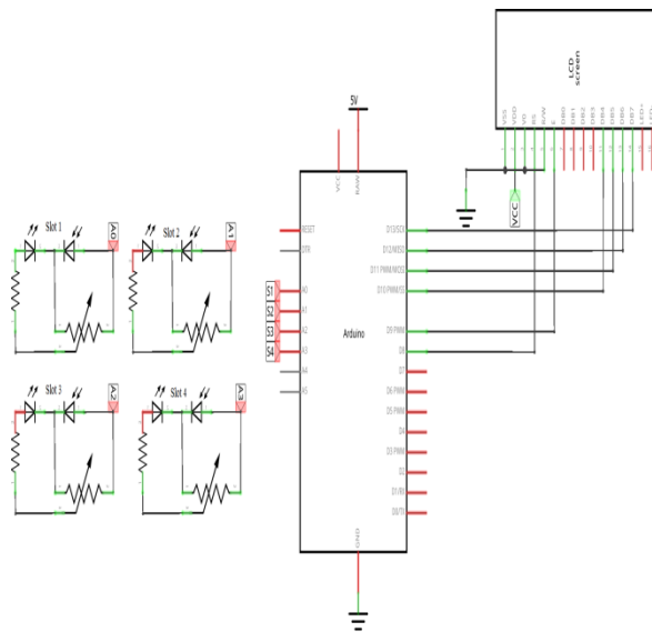
Fig:-5 Circuit diagram
