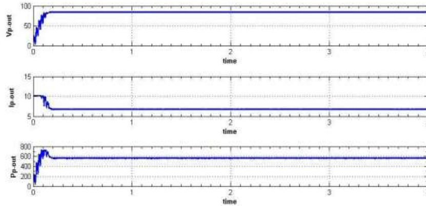
Fig 5.3.1 Voltage, current and power outputs of PV Panel
