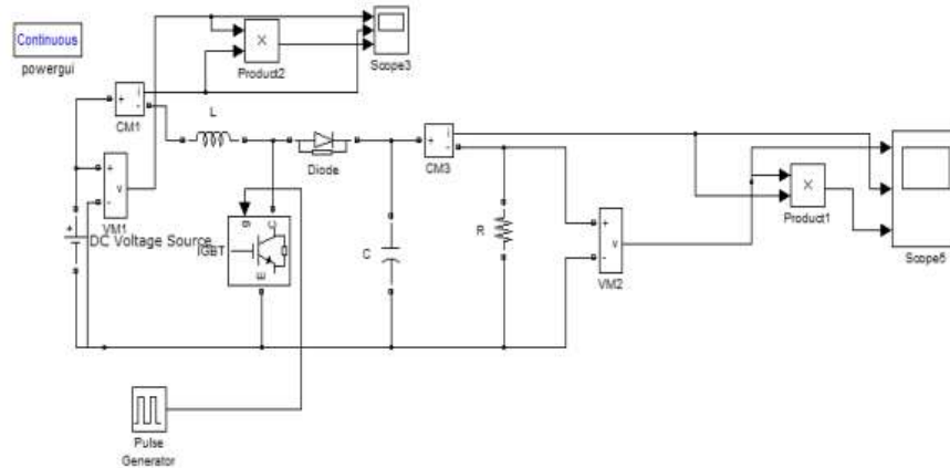
Fig 5.2 Simulation Results For Boost Converter
