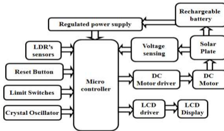
Fig 5.6.1 Block diagram of Hardware setup of proposed system
