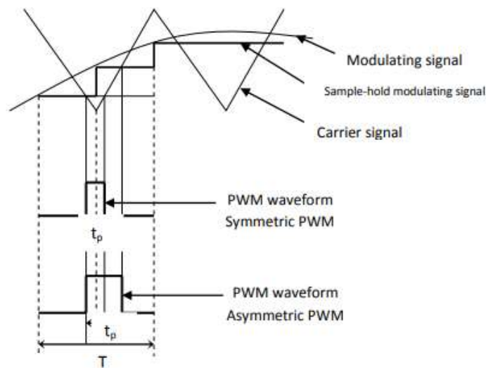
Fig.4.2 Details of symmetric and asymmetric PWM
