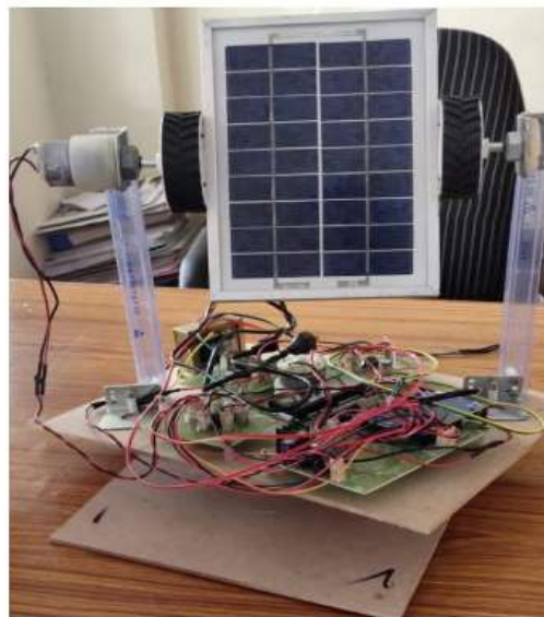
Fig 5.6.2 Hardware setup developed with dual axis tracking Solar panel
