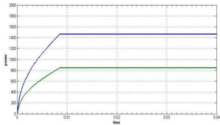
5.5.4 Active and Reactive power of inverter
