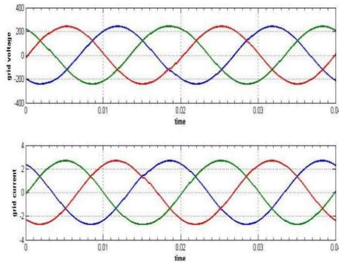
Fig 5.5.5 Output voltage and current of grid integration
