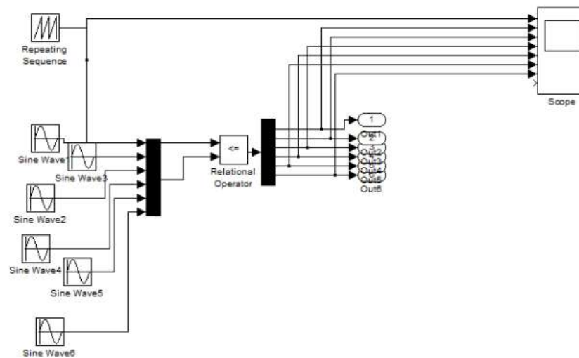
Fig 5.4.2 Simulink diagram of PWM Pulses
