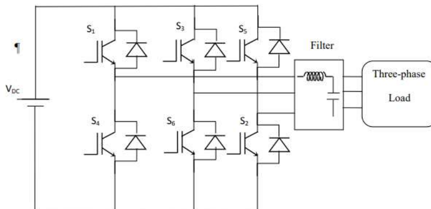
Fig:4.5 Three Phase Full-Bridge Inverter
