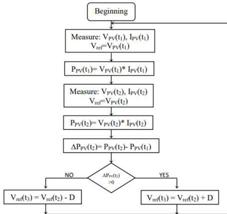
Fig:4.1 Flow chart for working model
