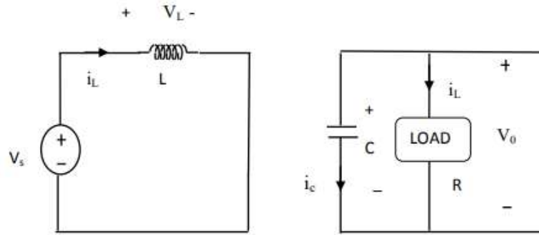
Fig 3.2 Mode 1 Operating Circuit
