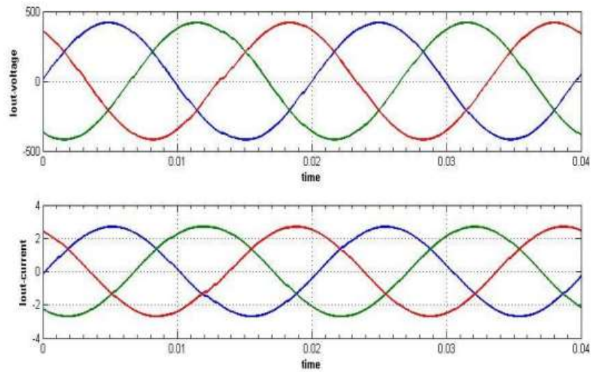
Fig 5.5.3 Output waveforms of inverter voltage and current
