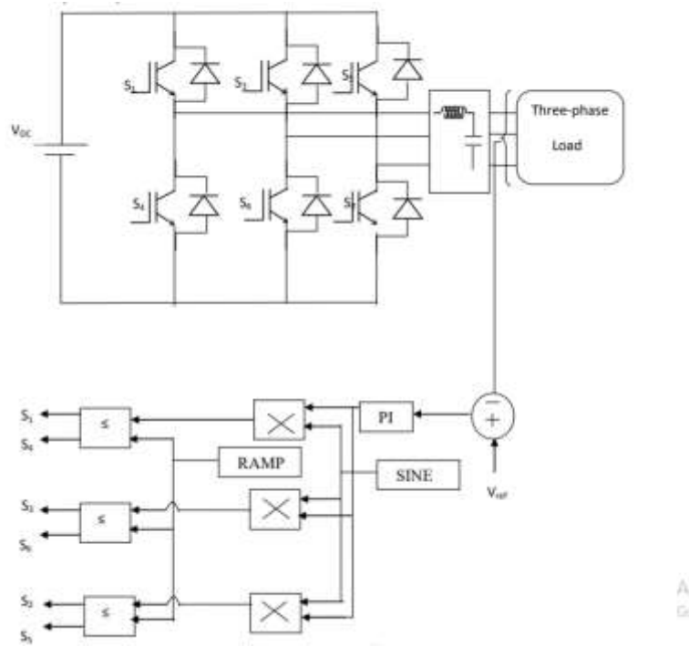
Fig:4.9 Control Strategy of Proposed Model
