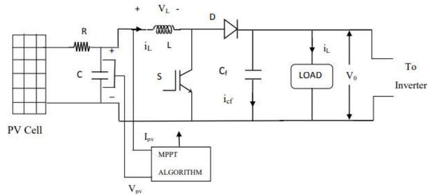
Fig. 2.7 Closed loop block diagram of solar powered Boost converter
