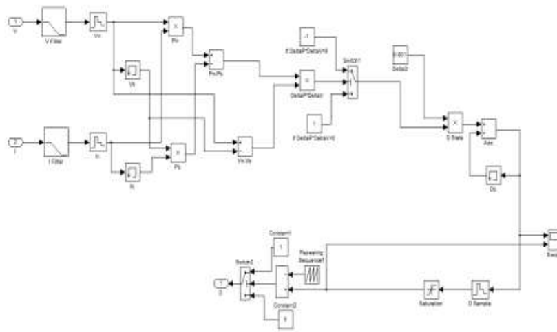
Fig 5.3.3 Simulink diagram of Maximum power point tracking by P & O method
