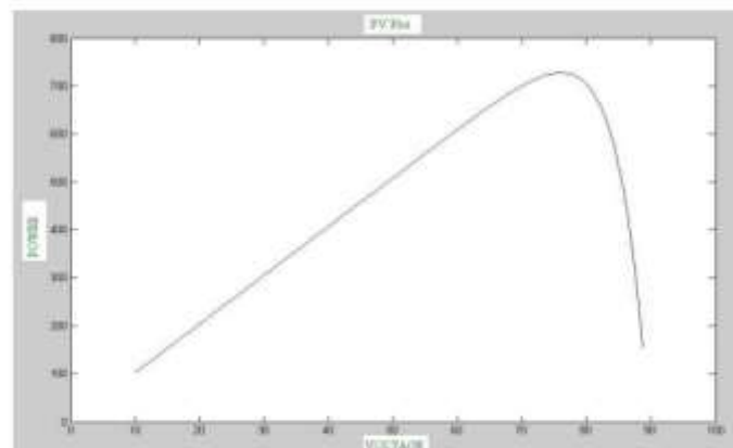
Fig 5.1.3 Plot of P-V
