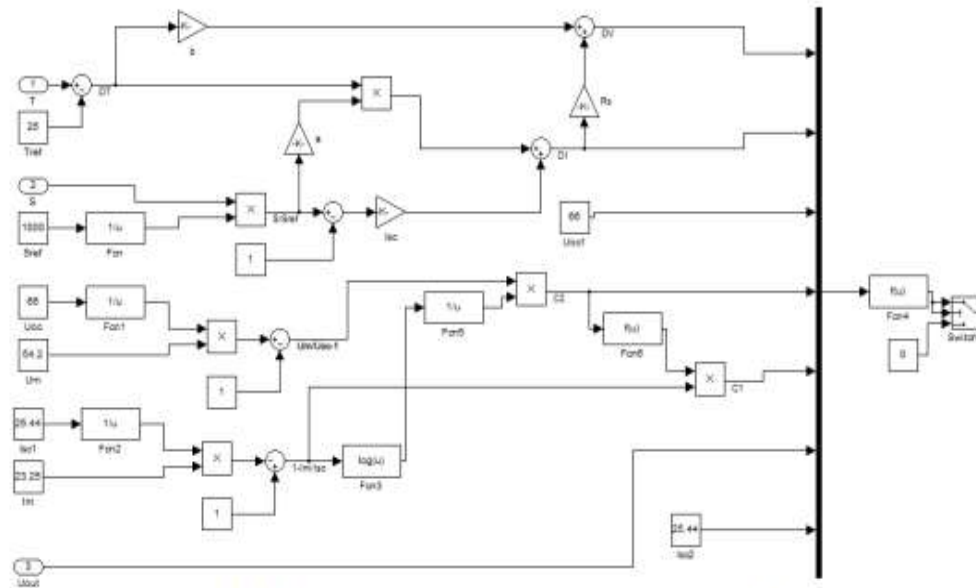
Fig 5.1.1 Unmasked block diagram of modeled solar PV panel
