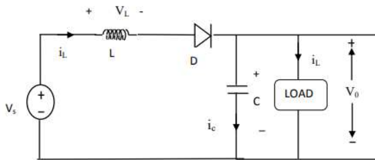
Fig 3.3 Mode 2 Operating Circuit
