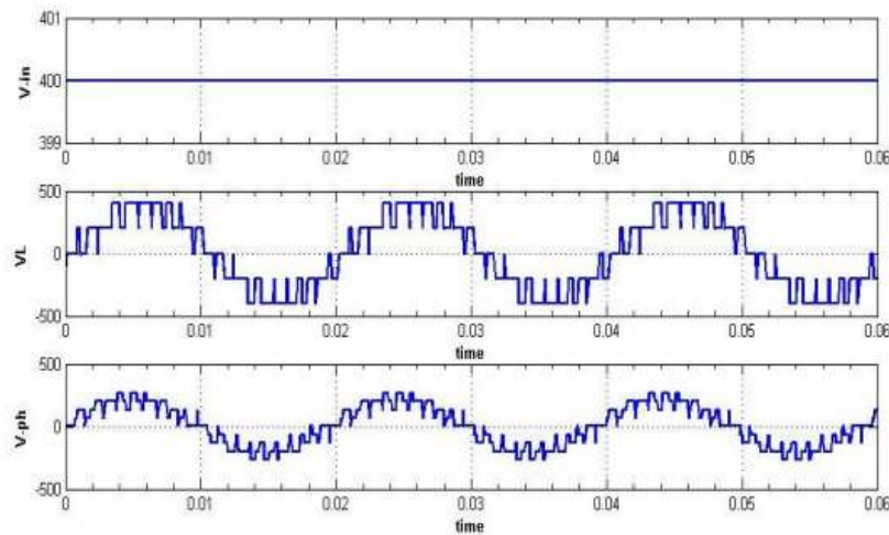
Fig 5.4.3 Input, Line, Phase voltages of SPWM Inverter
