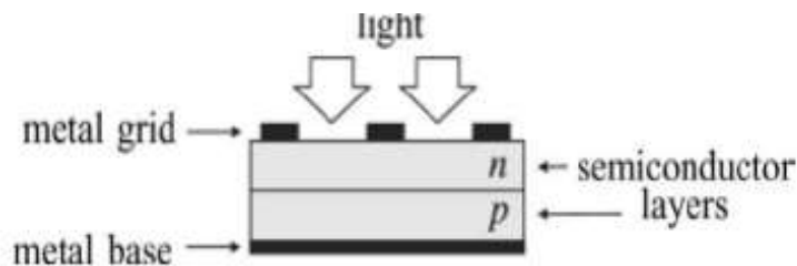
Fig 2.3: Physical structure of a PV cell
