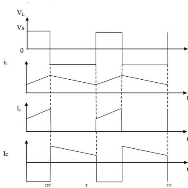
Fig 3.4 Waveforms of Current and Voltages
