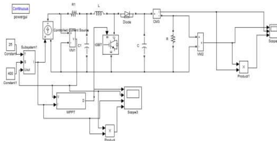
Fig 5.3(b) Simulink diagram of PV fed to Boost Converter with MPPT
