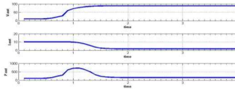
Fig. 5.1.2 Voltage, current and power outputs of a PV panel
