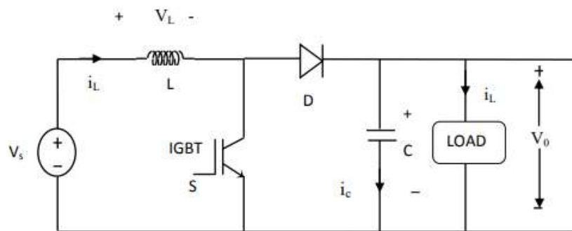
Fig 3.1 Basic DC-DC Boost Converter
