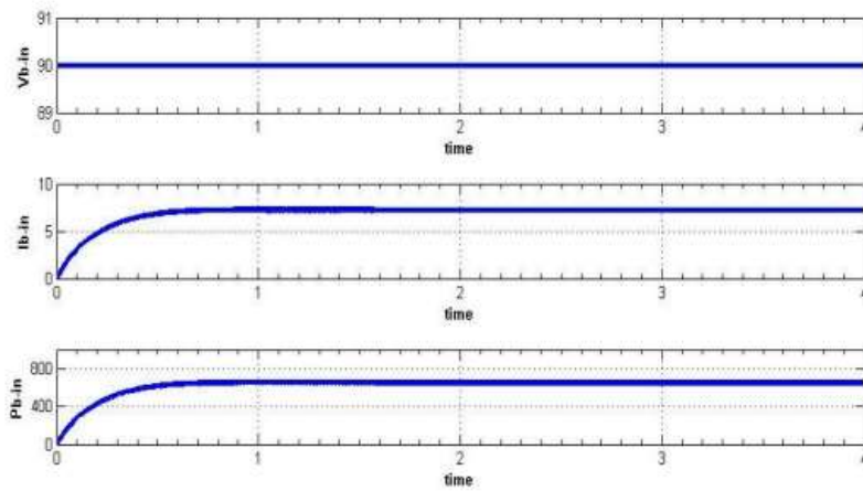
Fig.5.2.1 Voltage, current and power inputs of Boost converter
