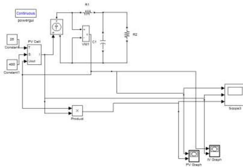
Fig.5.1 Simulink diagram of a PV Panel
