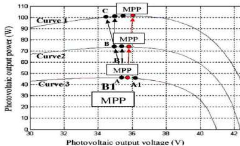
Fig :4.2 Photo voltaic output characteristics
