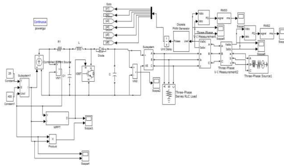
Fig 5.5 Simulink diagram of PV fed boost converter with 3-Ø Inverter to grid integration
