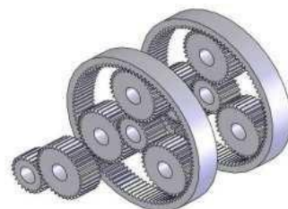
Fig 4a -Traditional Wind Turbine Gearbox
