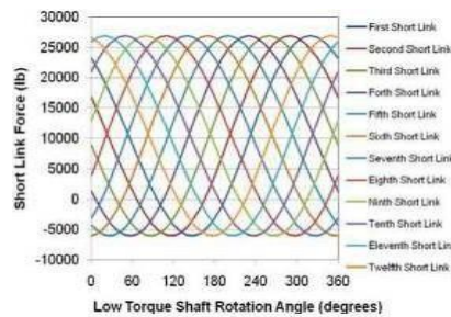
Fig 7 -Short Link Forces for One Rotation of the Low Torque Shaft
