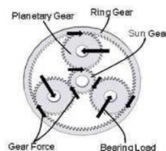
Fig 4b.-Planetary Gear Set Loads
