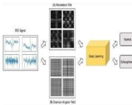
Figure 2. Image conversion and deep learning process of EEG data.
