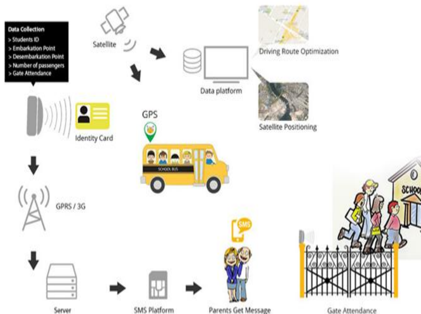
Figure 1. System architecture
