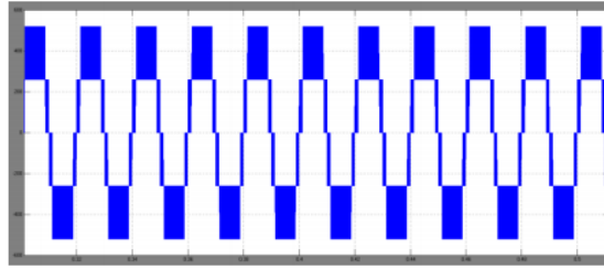
Fig15. STATCOM output voltage
