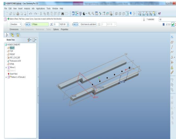
Figure 2. Channel with cross members using pattern
