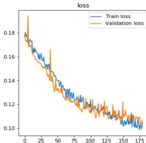
Figure 2: Learning curve of original kernel
