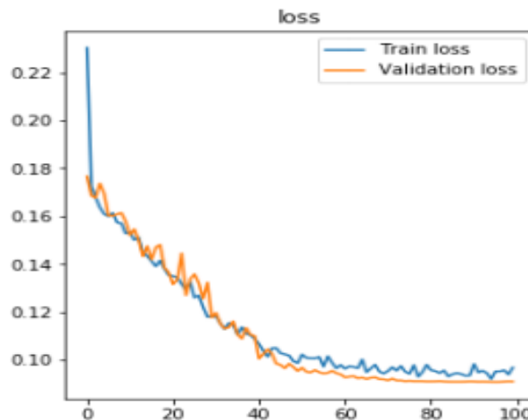
Figure 5: Learning curve of our model
