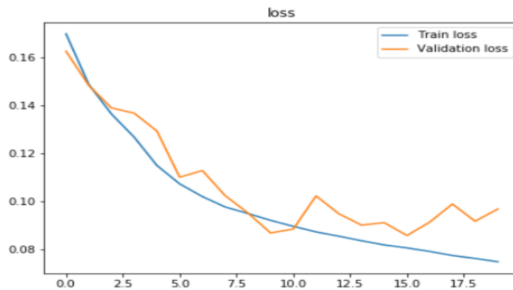
Figure 4: Learning curve of original kernel
