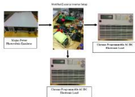
Fig. 15. Experimental setup
