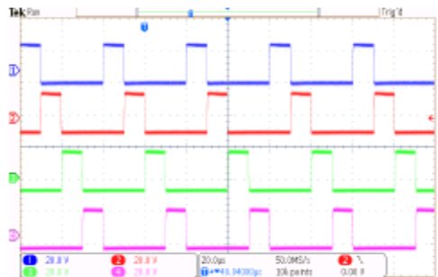
Fig. 12. PWM logic for the isolated HBC
