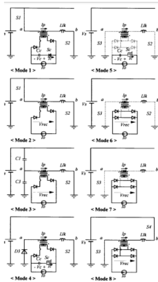
Fig. 2. Operation mode diagrams for eight modes. capacitor. So, the primary current is decreased as follows:
