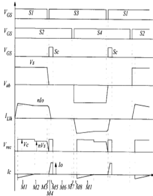
Fig. 3. Operation waveforms.
