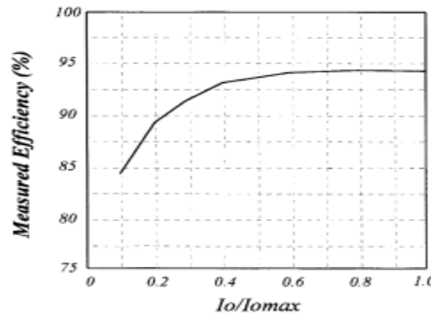
Fig. 14. Measured efficiencies.
