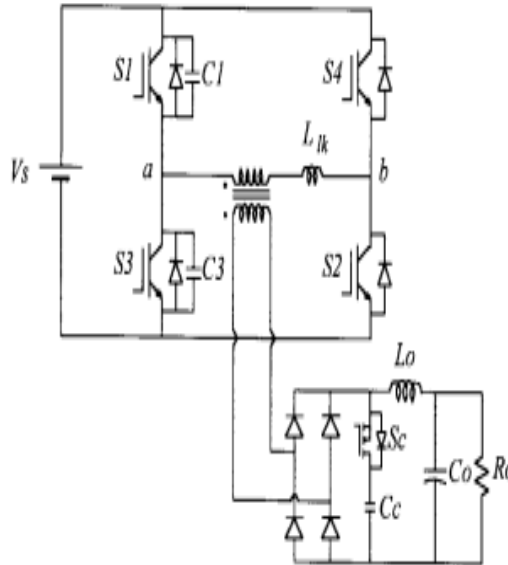
Fig. 1. Circuit topology of the proposed ZVZCS FB PWM converter.
