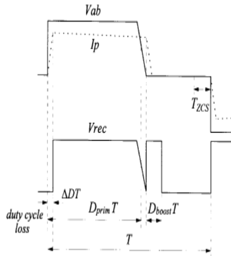
Fig. 5. Primary and secondary rectifier voltage waveforms.
