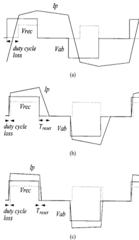
Fig. 4. Comparison of the simplified waveforms of primary voltages and currents and secondary rectifier voltages. (a) ZVS PWM converter. (b) ZVZCS PWM converters [7], [8]. (c) Proposed converter.
