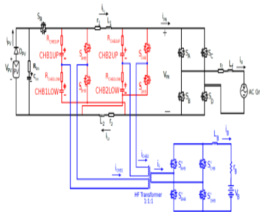
Fig. 2. Detailed Schematic of Proposed MZSI
