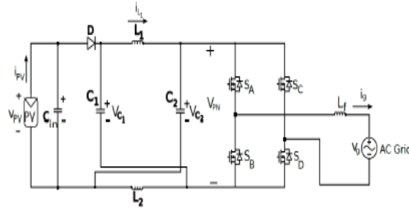
Fig. 1. Schematic of a Photovoltaic/AC grid inter- connected Z-source Inverter(ZSI)
