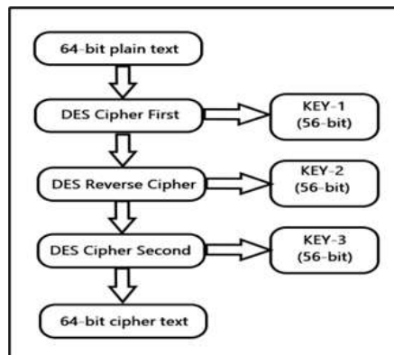
Fig.7. Triple-DES Algorithm
