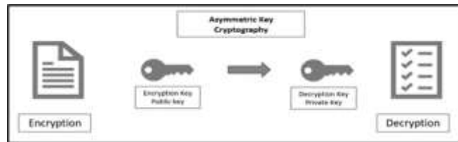
Fig.4. Asymmetric Algorithm
