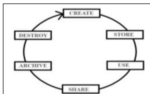
Fig.1. Data Lifecycle
