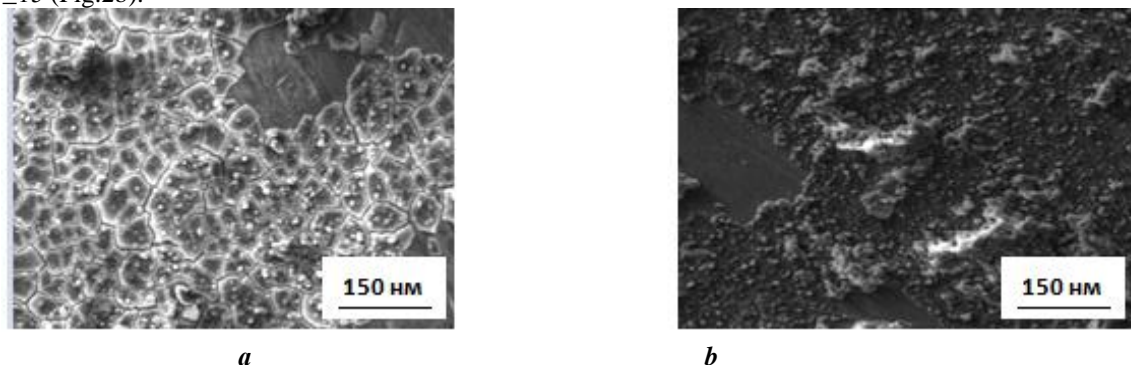
Fig.2: Composite nanocoatings \text{FB}_1 (a) and \text{FB}_2 (b) on the surface of the titanium electrode
