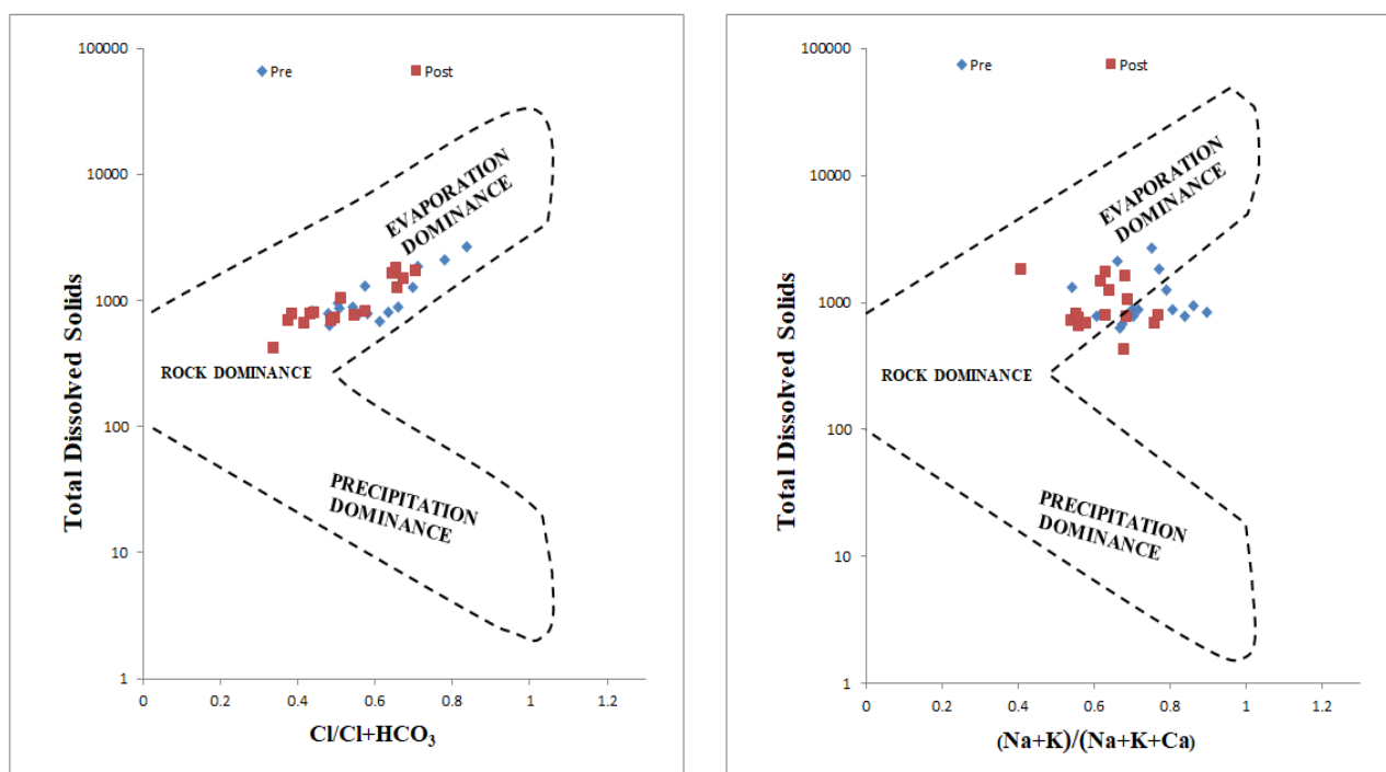
Figure 5: Gibbs diagram showing the mechanisms influencing the groundwater chemistry
