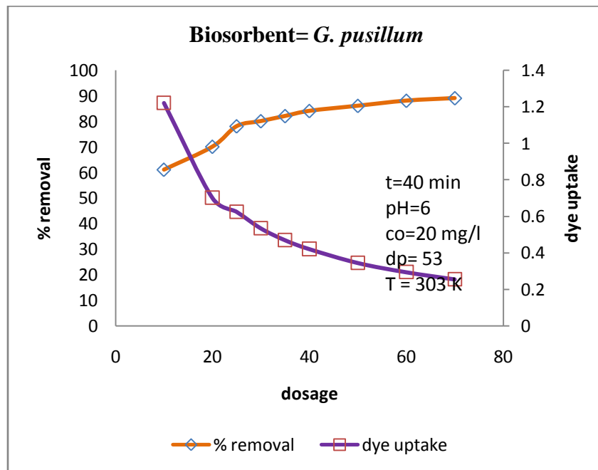
Fig. 3.3. Effect of biosorbent dosage on % biosorption of CV dye
