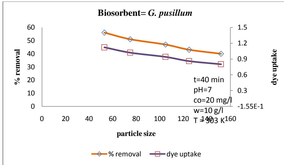
Fig. 3.2. Effect of biosorbent size on % biosorption of CV dye
