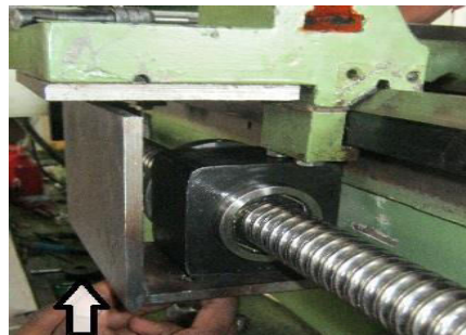
Fig.7 Z-axis ballscrew attached on main slide
