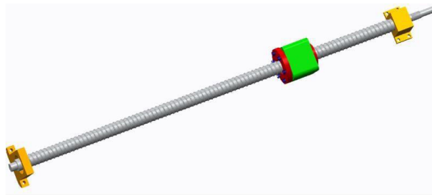
Fig.6 Assembly of Z-axis ballscrew with bracket
