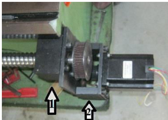
Fig.8Z-axisMountingbracket&Steppermotor
