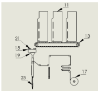
Figure 8. Side view of the assembly
