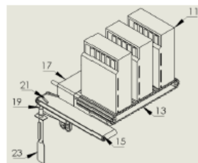
Figure 7. Total assembly of the machine
