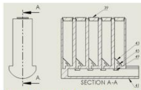
Figure 5. Cross sectional view of the receptacle Referring now to figure 3 and 4, the storage space contains a number of receptacles. Each receptacle
