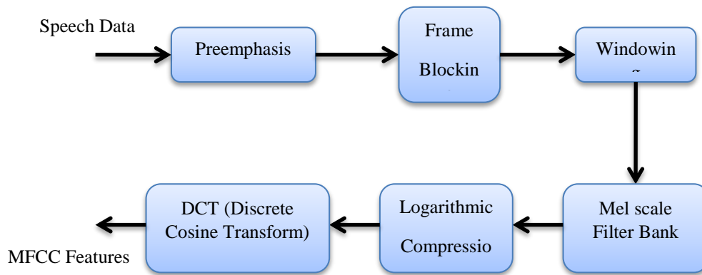
Figure 2. MFCC operation diagram
