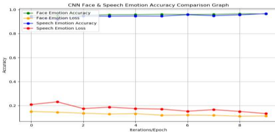
Figure 8: Accuracy and loss comparison of proposed CNN with speech and facial expression.
