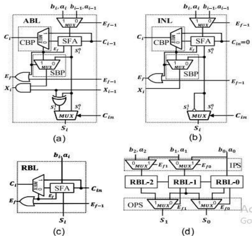
Figure 3. Fundamental blocks for constructing the self-repairing HA using (a) ABL (b) INL (c) RBL for CSeA and RCA block along with the shifting approach (d) for input and Sum-out in case of fault detection.
