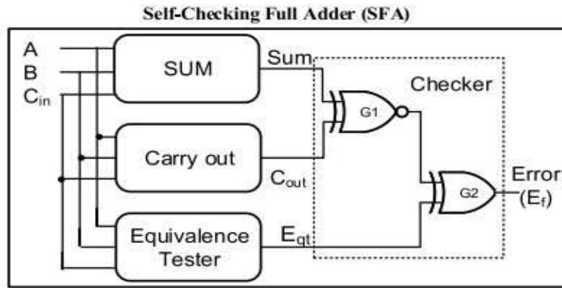
Figure 1. Block Diagram of Self Checking Full Adder
