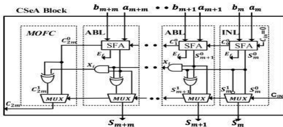
Figure 2. Block diagram of Carry select adder (CSeA)
