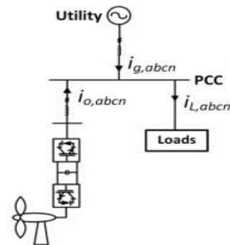
Fig. 5 Single line diagram of the addressed industrial system with wind turbine system.
