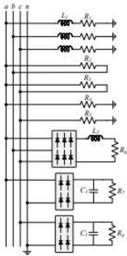
Fig. 8 Configurable load
