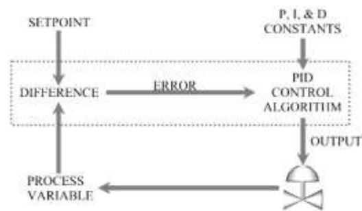
Fig.1 PID working module
