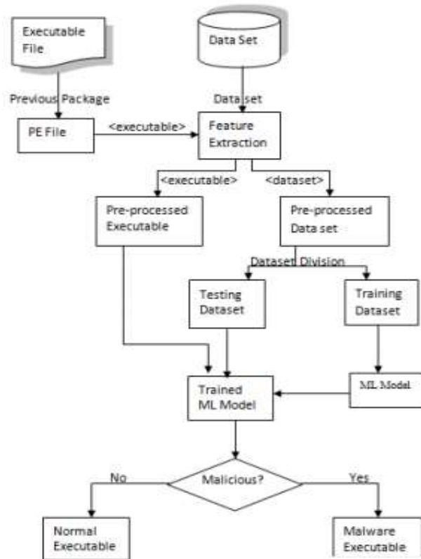
Figure 1: System Architecture
