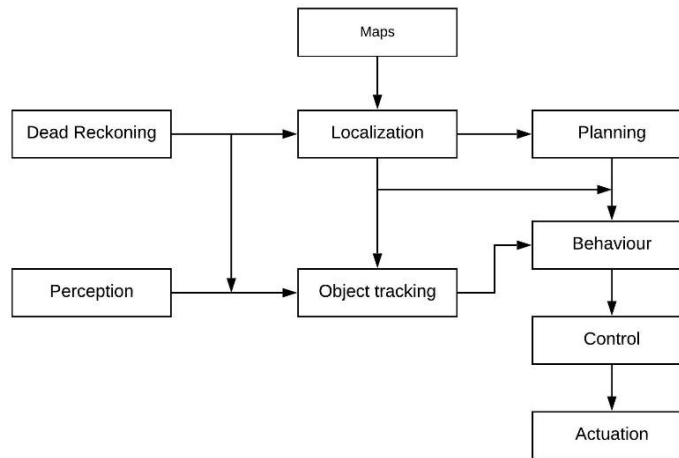
Fig.2. Block diagram of Localization and control system
